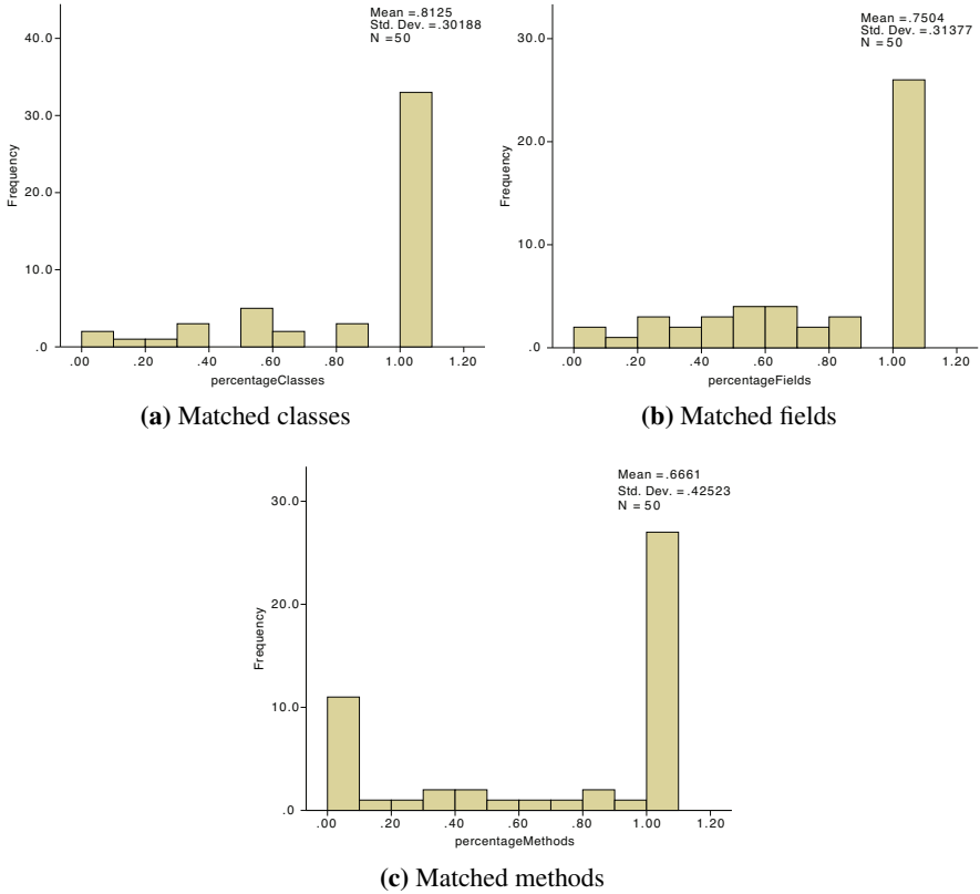
Fig. 11. Histogram of correctly matched classes (a), fields (b), and methods (c)
