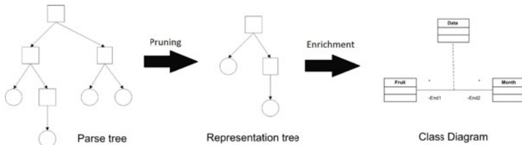
Fig. 5. Overview of the Transformation step to transform a parse tree into a class diagram
