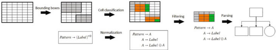
Fig. 4. Overview of the pattern recognition process
