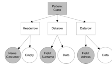
Fig. 7. Parse tree generated for the Customer spreadsheet
