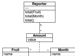
Fig. 2. Class diagram extracted from the fruit example
